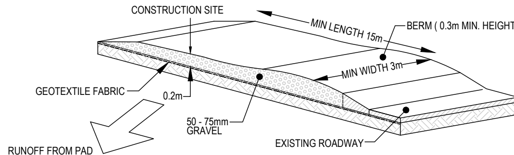
STABILIZED SITE ACCESS NTS
