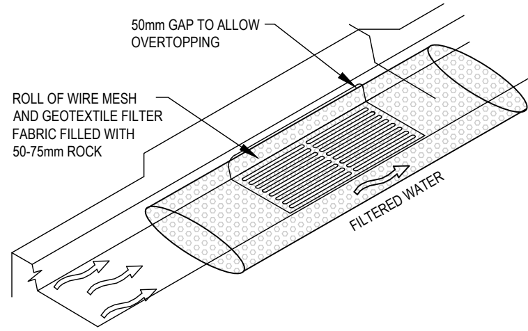
MESH AND GRAVEL INLET FILTER NTS
