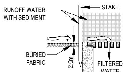
SEDIMENT BARRIER AROUND PIT NTS
